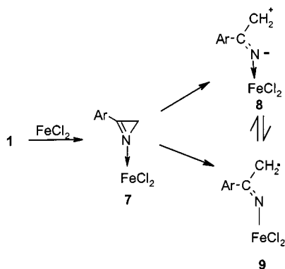
Scheme 2. Formation of the azirine-FeCl 2 complex
